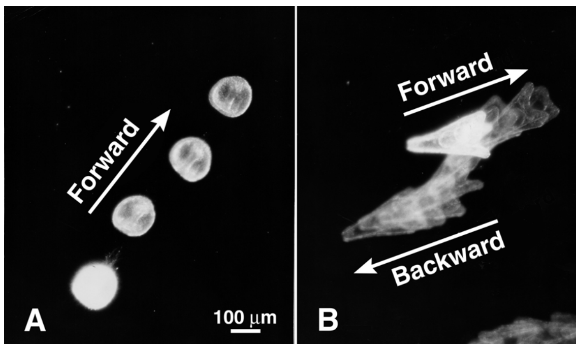
Fig. 1. Multiple-exposure photographs of swimming embryos of the sea urchin, Hemicentrotus pulcherrimus . A: gastrula stage; B: pluteus stage. Exposure intervals: 1 s (A) and 2 s (B); the brightest images are made by the first flash of stroboscopic exposure. 12 °C.
